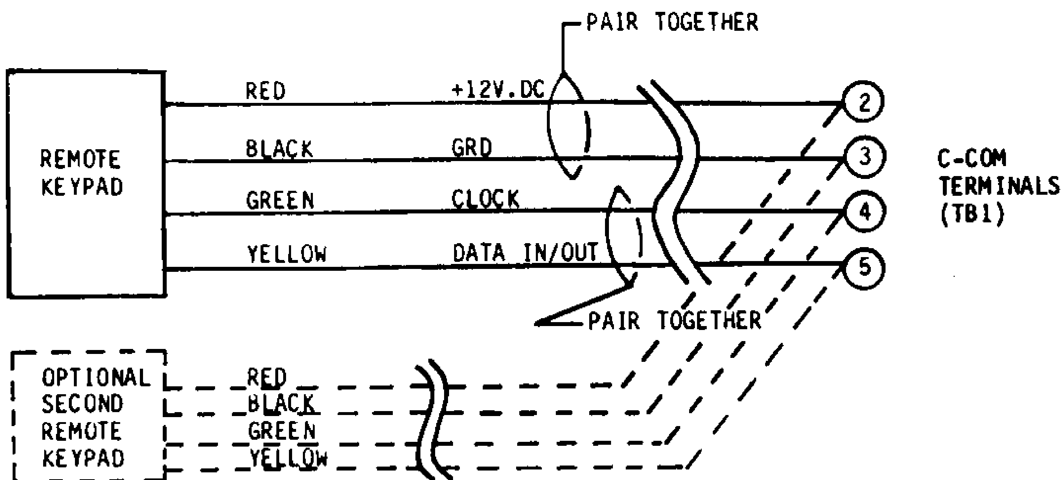
Diagram 1: KEYPAD CONNECTIONS
