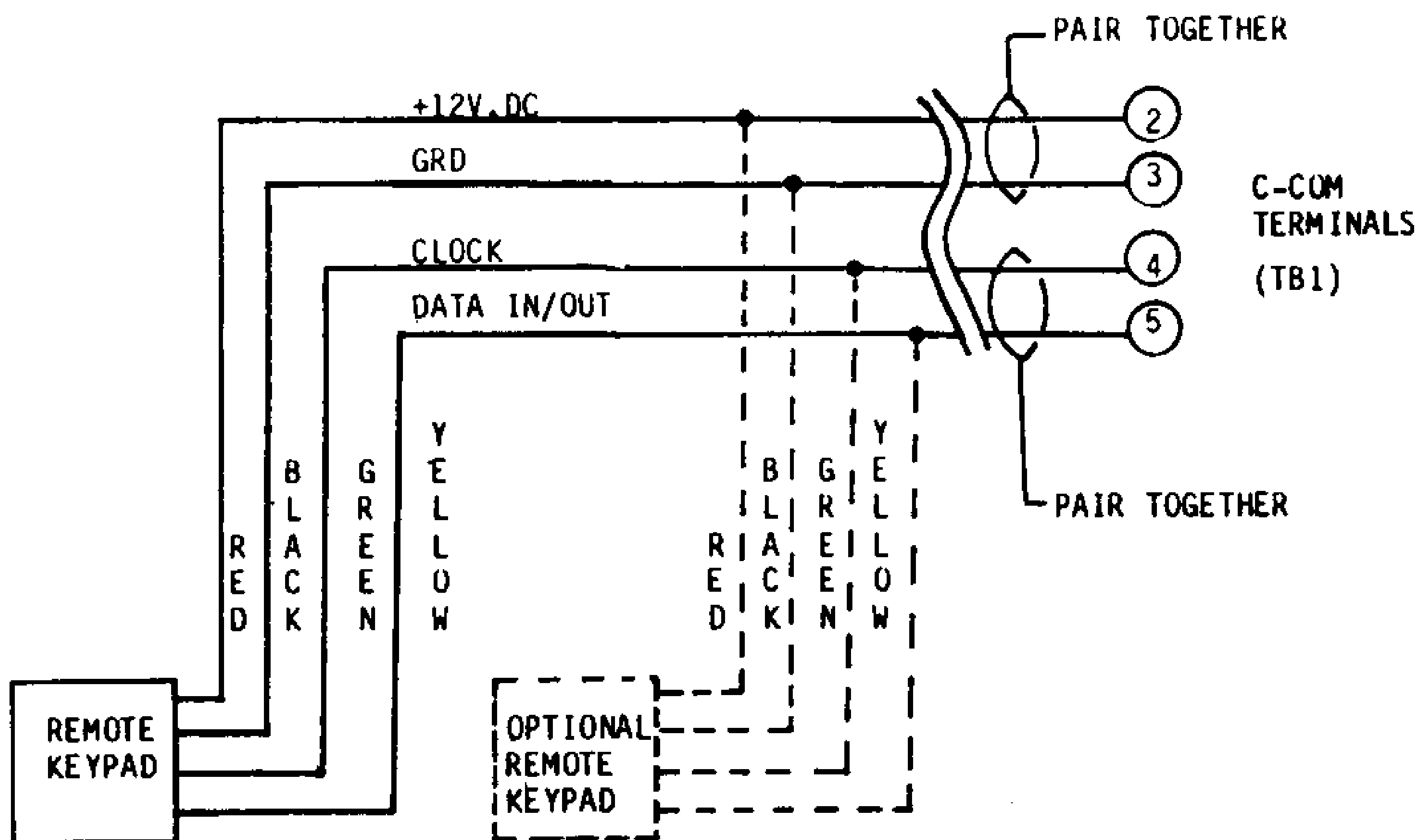
Diagram 2: KEYPAD CONNECTIONS
