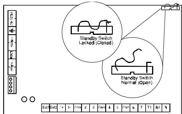
Figure 2: Standby Switch
