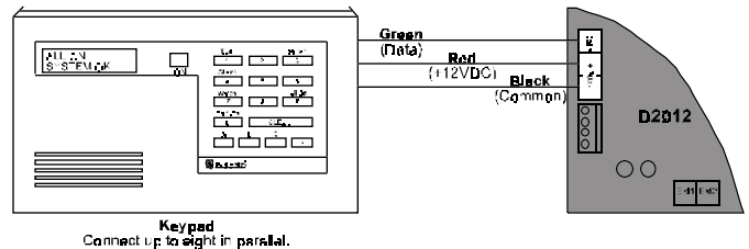
Figure 3: Keypad Wiring
