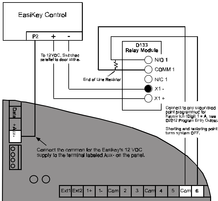
Figure 13: Keyswitch
