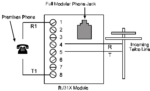
Figure 6: RJ31X Phone Jack
