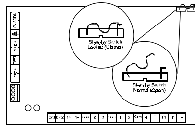
Figure 8: Standby Switch
