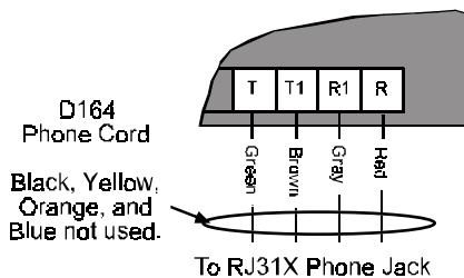
Figure 7: Phone Cord
