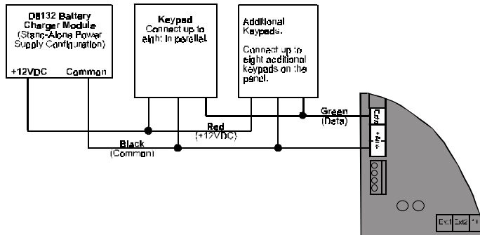
Figure 10: Power for Keypads
